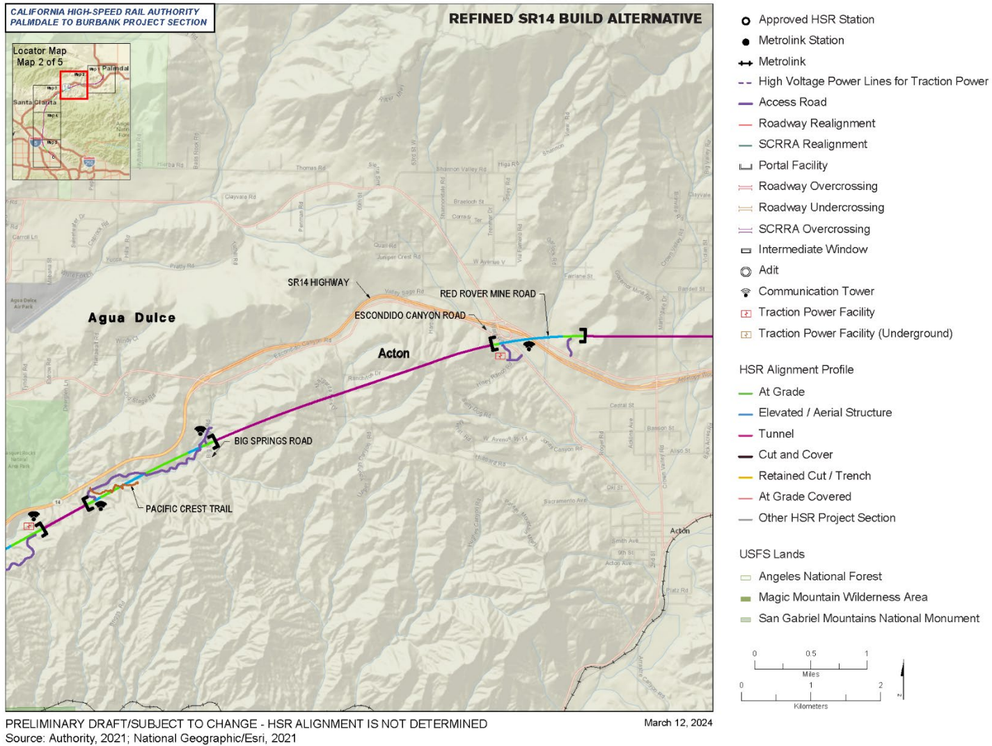
Figure 2-50 Refined SR14 Build Alternative (Map 2 of 5)
