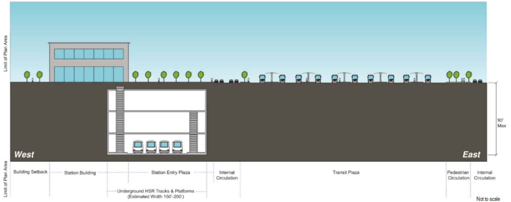
Figure 2-55 Burbank Airport Station Preliminary Station Concept Layout Plan—Cross Section
