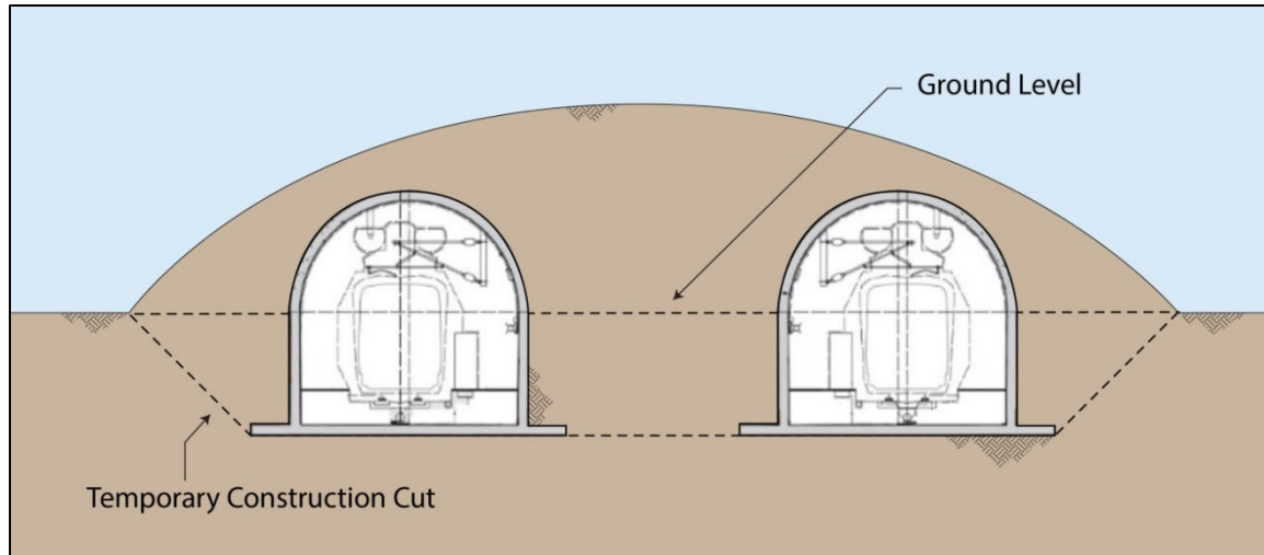
Figure 2-13 Typical High-Speed Rail At-Grade Covered Tunnel Cross Section
