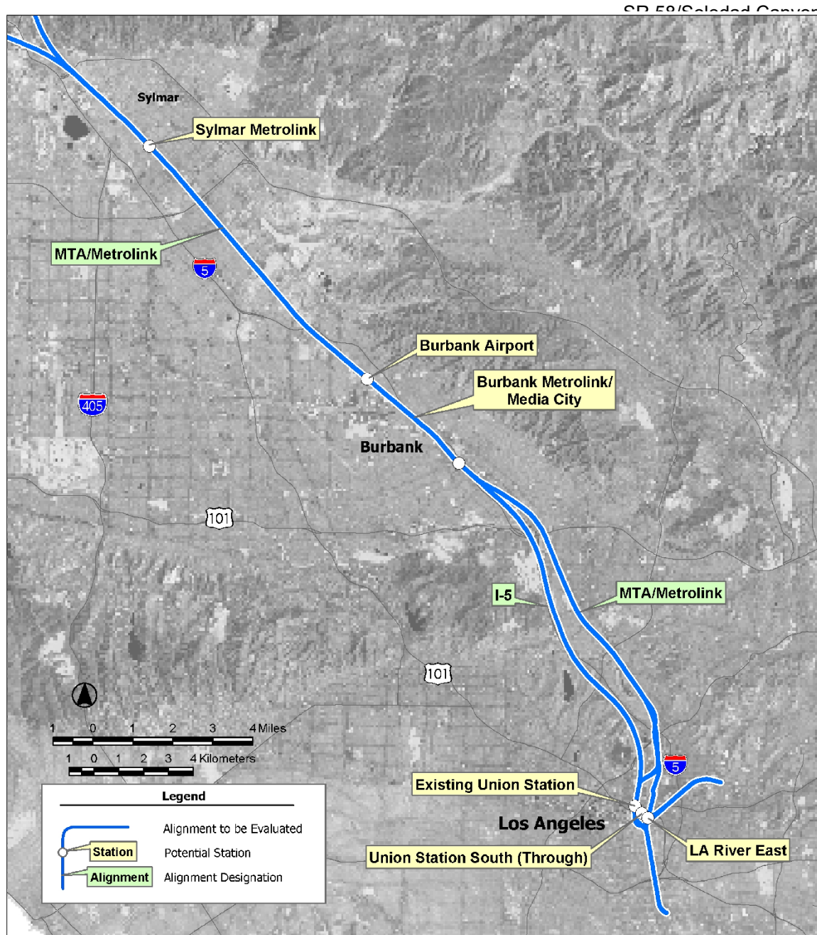
Figure 2-33 Sylmar to Los Angeles Corridor Alignments and Station Sites Carried Forward
